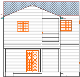
PLAN DE FACADE PRINCIPALE
